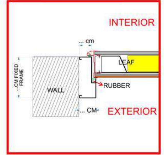
FIXED FRAME
