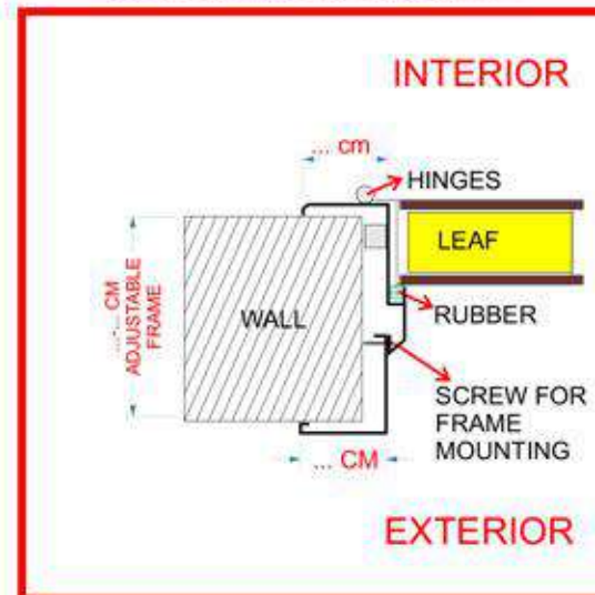
EXTERNAL SCREWED ADJUSTABLE FRAME
