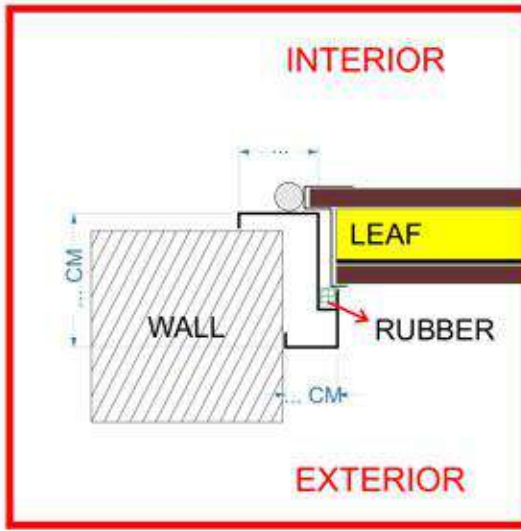
INTERNAL MOUNTED FIXED FRAME
