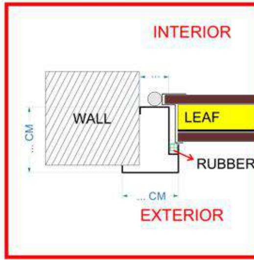
EXTERNAL MOUNTED FIXED FRAME
